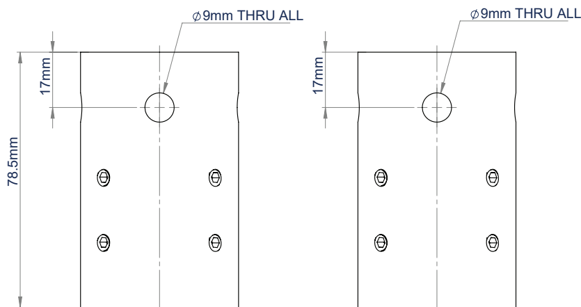
VISTA FRONTAL
