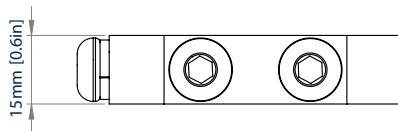
FRONT VIEW - WITHOUT COVER
