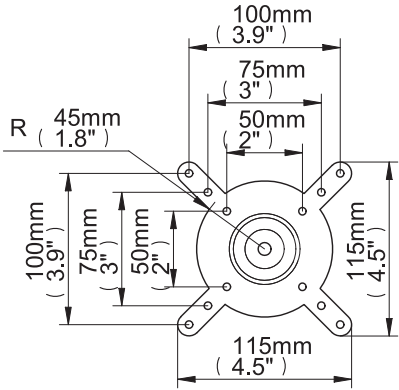
INTERFACE PLATE
