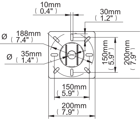
CEILING PLATE
