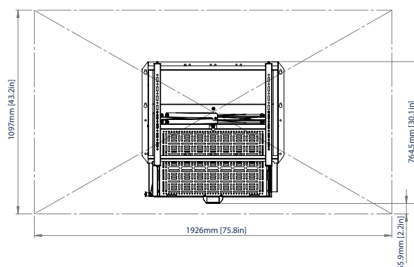
86" SCREEN - CLOSED
