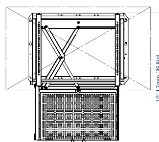
49" SCREEN - OPEN
