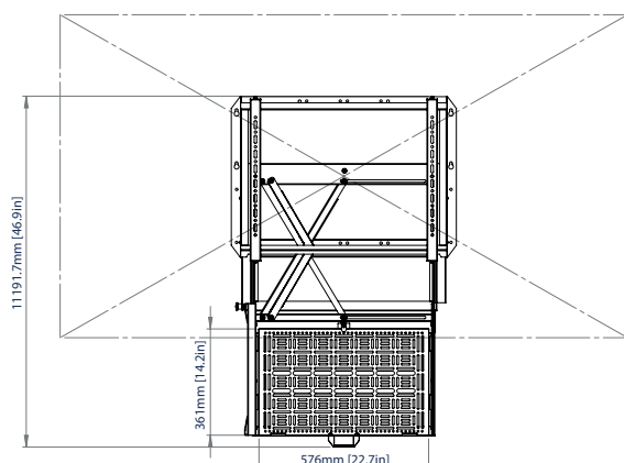
86" SCREEN - OPEN
