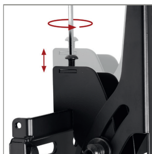
Arms feature leveling screws to adjust the screen height once mounted
