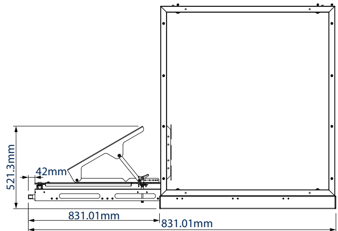
SIDE VIEW TRAY EXTENDED
